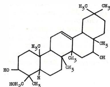
Sojasapogenol B
