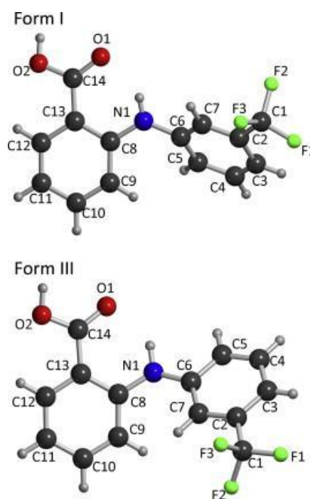
Figure 3. Models of two flufenamic acid polymorphs, the form I and III (Delaney et al., 2014).
