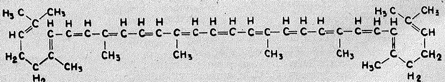
likopin
