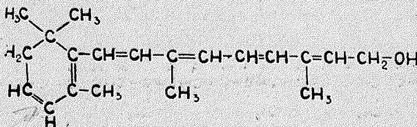
vitamin A 2
