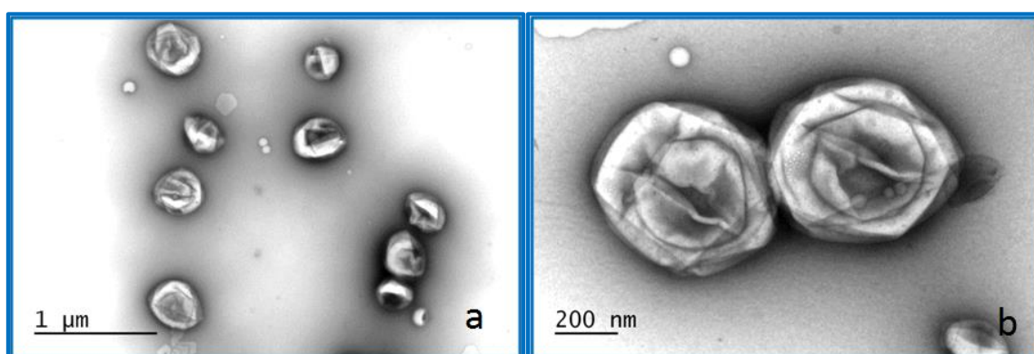
Figure 24. TEM images of PDMS 65 -b-PMOXA 14 Ps prepared using the film rehydration technique and extrusion through 200 nm filters. Scale bars used are 1 μm and 200 nm.
