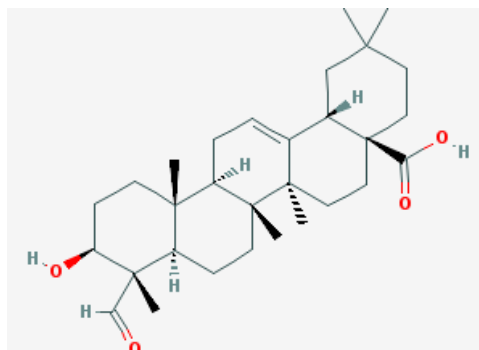
Gipsogenin
