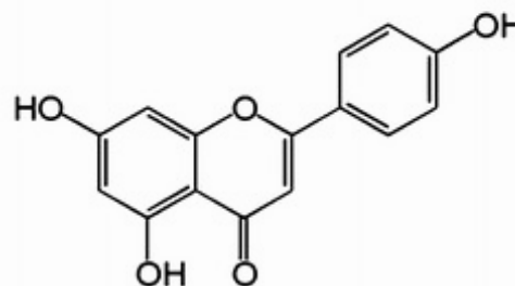
Apigenin
