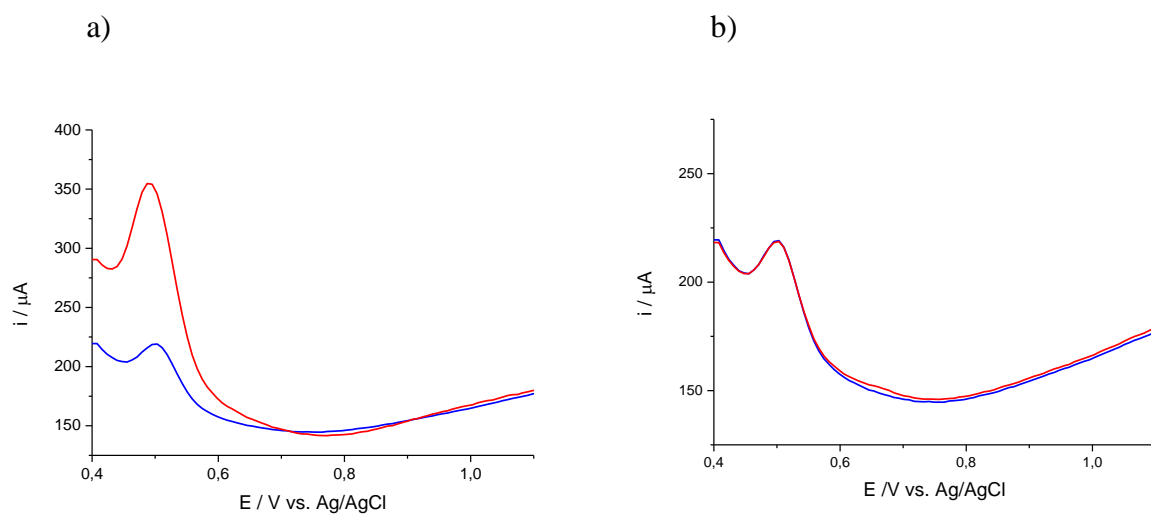
Supplementary Figure 7. Square-wave voltammograms of L-dopa ( 1 \times 10^{-6} M) at the MWCNTs/Nafion-GCE: (a) with equal DA concentration (red) and without DA (blue). (b) with plasma concentration (26 pg/mL) of DA (red) and without DA (blue). SWV settings: f = 50 Hz, E_{\text{sw}} = 25 mV and \Delta E = 8 mV ( E_{\text{acc}} = 0 V, t_{\text{acc}} = 240 s)
