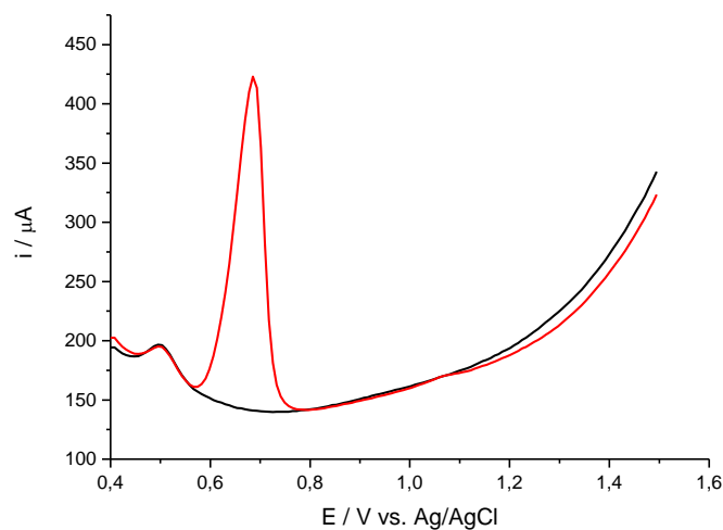
Supplementary Figure 8. Square-wave voltammograms of L-dopa ( 1 \times 10^{-6} M) at the MWCNTs/Nafion-GCE with 50-fold uric acid (red) and without uric acid (black). SWV settings: f = 50 Hz, E_{\text{sw}} = 25 mV and \Delta E = 8 mV ( E_{\text{acc}} = 0 V, t_{\text{acc}} = 240 s)
