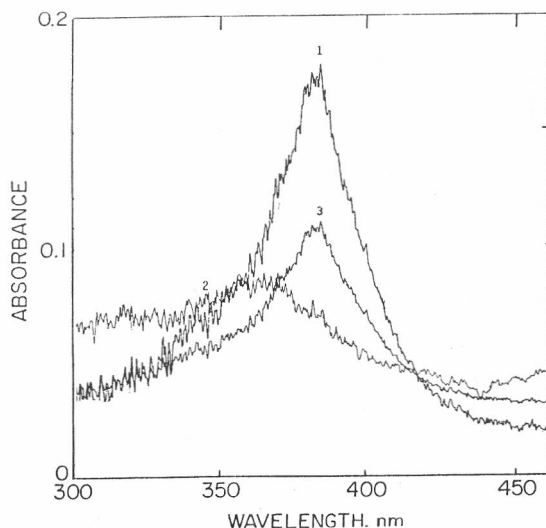
Figure 3. Rapid-scan low-temperature stopped-flow study of the reaction of 1.5 \mu\text{M} ferri-DFH with 3.2 mM m -CPB in 10 mM phosphate containing 1% v/v 1,2-dimethoxyethane ( I = 0.1 \text{ M NaCl} ) at pH 5.5 at 0 ^{\circ}\text{C} . Curves 1–3 are spectra of ferri-DFH and the intermediates present 5 s and 5 min after the start the reaction, respectively.
