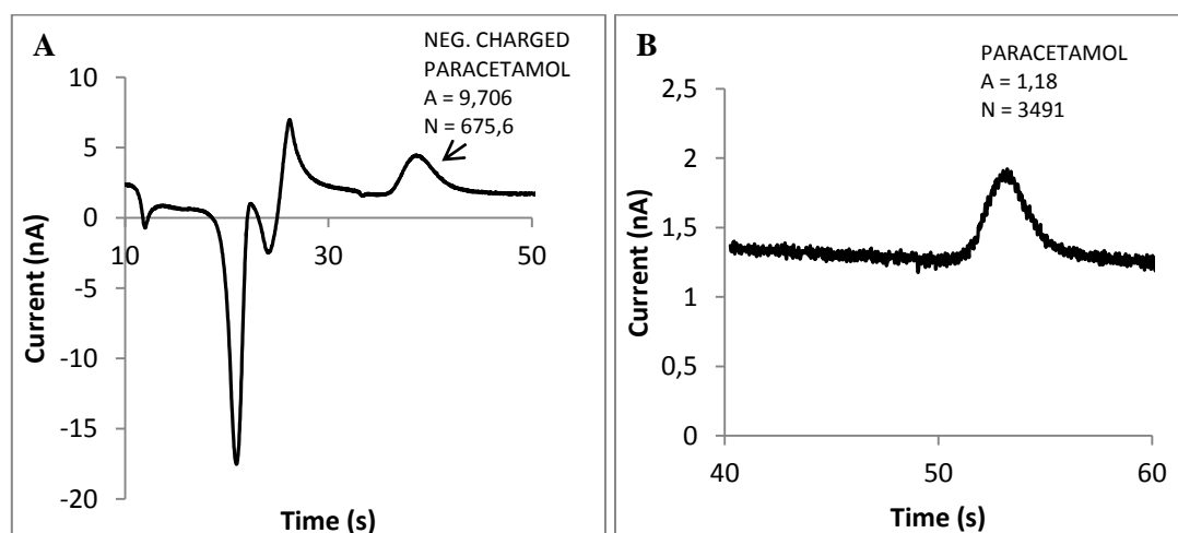
Figure 15. Electropherograms of paracetamol 50 \mu\text{M} with electrokinetic sample stacking with 10 mM sodium borate pH 10.0 as a sample buffer and 100 mM sodium borate as running buffer (A); and paracetamol 50 \mu\text{M} without sample stacking with 100 mM sodium borate pH 10.0 as running buffer (B). Other conditions: V_{\text{sep}} = +1000 V, V_{\text{inj}} (A) 800 V for 24 s (gated C \rightarrow B injection); V_{\text{inj}} (B) +800 V for 6 s (C \rightarrow D injection), E_d = +0.9 V. L_{\text{eff}} = 30 mm.
