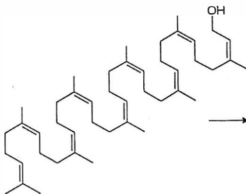
Solanesol
