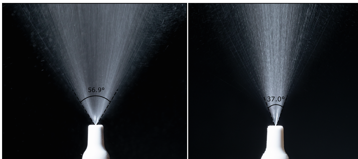
Fig. 5. Spray cone angles of in situ gelling fluticasone (0.05%, w/w) suspensions prepared with (a) pectin (0.05%, w/w; sample 9) and (b) pectin and gellan gum (0.05% and 0.2%, w/w, respectively; sample 15).
