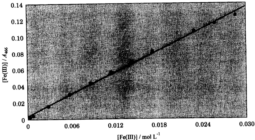
Figure 3. Dependence of Fe(III)/ A_{466} on iron(III) concentration. [HA \text{ unit}] = 2.95 \times 10^{-4} \text{ mol L}^{-1} ; [HClO_4] = 0.10 \text{ mol L}^{-1} ; I = 2.00 \text{ mol L}^{-1} (H/NaClO 4 ); t = 25 \text{ }^\circ\text{C} .
