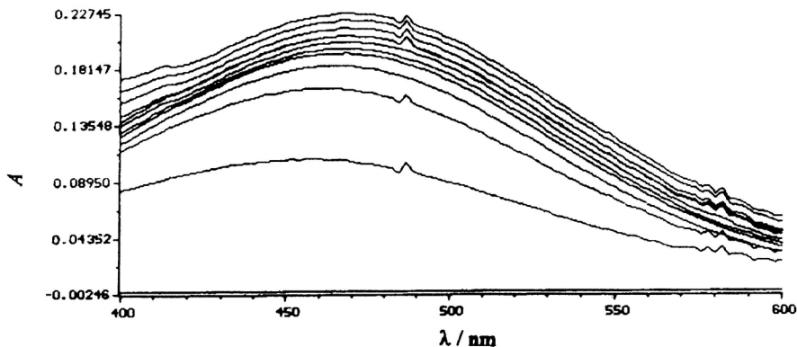
Figure 4. Absorption spectra of the PHA-Fe(III) system at different iron(III) concentrations [HA \text{ unit}] = 3.00 \times 10^{-4} \text{ mol L}^{-1} ; [HClO_4] = 0.10 \text{ mol L}^{-1} ; [Fe(III)] = 2.860 \times 10^{-4} (the lowest curve), 7.150 \times 10^{-4} , 2.859 \times 10^{-3} , 5.718 \times 10^{-3} , 8.577 \times 10^{-3} , 1.144 \times 10^{-2} , 1.429 \times 10^{-2} , 1.715 \times 10^{-2} , 2.287 \times 10^{-2} , 2.573 \times 10^{-2} , 2.859 \times 10^{-2} \text{ mol L}^{-1} (the highest curve); I = 2.00 \text{ mol L}^{-1} (H/NaClO 4 ); t = 25 \text{ }^\circ\text{C} .
