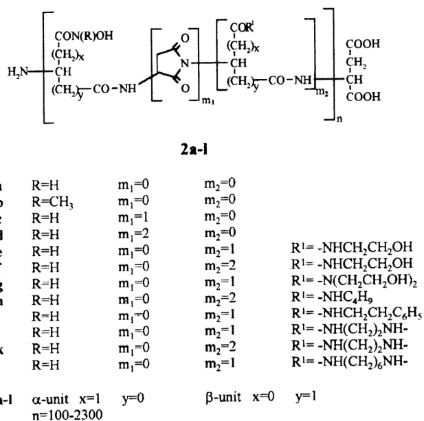
Figure 1. Structure of polyhydroxamic acids 2a-l .
