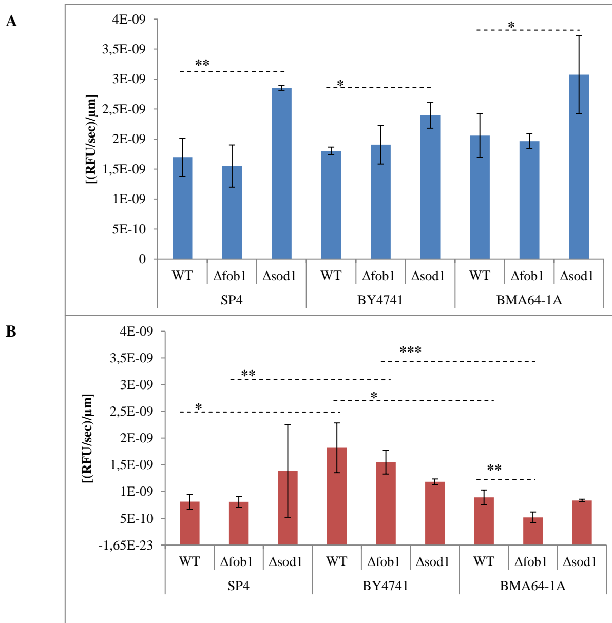
Figure 14. The ROS concentration normalized per cell size at exponential (A) and stationary (B) phase of cell growth. The results are presented as relative fluorescence units per second (RFU/sec/µm) and expressed as mean value \pm standard deviation. Three different S. cerevisiae strains (i.e. WT, \Delta fob1 , \Delta sod1 ) of three different genetic backgrounds (i.e. SP4, BY4741, BMA64-1A) were used in these experiments. * P < 0.05 ; ** P < 0.01 ; *** P < 0.001 ; **** P < 0.0001
