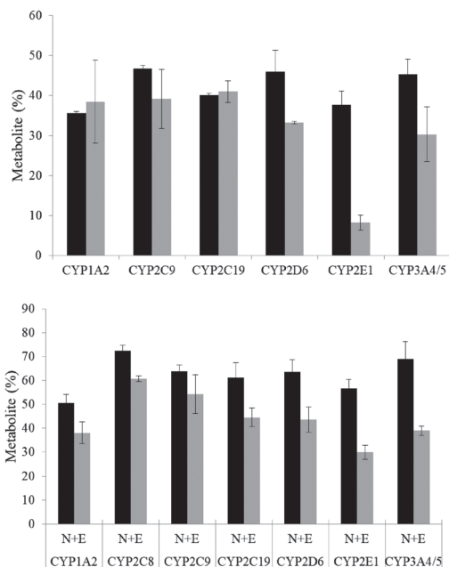
Fig. 4. Inhibition assays for the reactions: a) 3,7-dihydroxyflavone \rightarrow 3,7,4'-trihydroxyflavone and b) sakuranetin \rightarrow naringenin (N) + eriodictyol (E). Black columns represent the percentage of metabolite/s generated in control without the specific inhibitor of cytochrome P450 and grey columns with the addition of the inhibitor. Results represent the mean \pm standard error ( n = 3 ).
