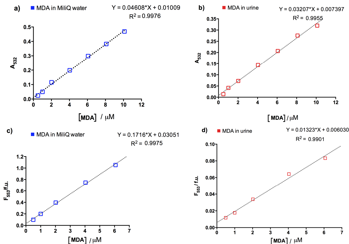
Figure 4. Calibration curves of MDA standard: spectrophotometric determination ( \lambda = 532 \text{ nm} ) in MilliQ water (a); spectrophotometric determination ( \lambda = 532 \text{ nm} ) in urine (b); spectrofluorometric determination ( \lambda_{\text{em}} = 553 \text{ nm} ( \lambda_{\text{ex}} = 515 \text{ nm} )) in MilliQ water (c); spectrofluorometric determination ( \lambda_{\text{em}} = 553 \text{ nm} ( \lambda_{\text{ex}} = 515 \text{ nm} )) in urine (d). Linear regression parameters are given on each plot.
