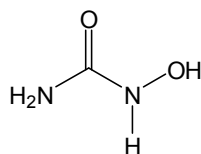
Figure 1. Chemical structure of hydroxyurea, noted as HU.
