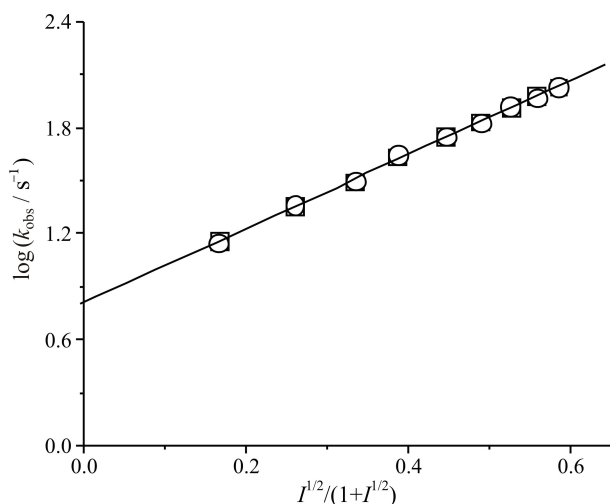
Figure 11. Dependence of \log k_{\text{obs}} on I^{1/2}/(1+I^{1/2}) . Conditions: [\text{Na}_3\text{Fe}(\text{CN})_6] = 0.5 \text{ mol dm}^{-3} , [\text{HU}] = 15 \text{ mmol dm}^{-3} , \text{p}[\text{H}^+] = 12.0 , \theta = (25 \pm 0.1)^\circ\text{C} . Ionic strength maintained with \text{NaClO}_4 (squares) and \text{NaNO}_3 (circles).
