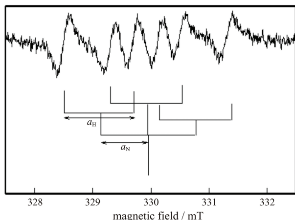
Figure 4. EPR spectrum of the aminocarbonylaminooxyl radical ( \text{H}_2\text{N}-\text{CO}-\text{NHO}^\bullet ). Conditions: [\text{HU}] = 0.1 \text{ mol dm}^{-3} , [\text{Fe}(\text{CN})_6^{3-}] = 0.01 \text{ mol dm}^{-3} , [\text{HClO}_4] = 0.01 \text{ mol dm}^{-3} , at room temperature with f = 9.28 \text{ GHz} and 10 \text{ mW} .
