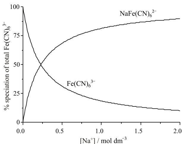
Figure 12. Distribution diagram of 5 \text{ mmol dm}^{-3} hexacyanoferrate(III) species as function of [\text{Na}^+] at 25^\circ\text{C} .
