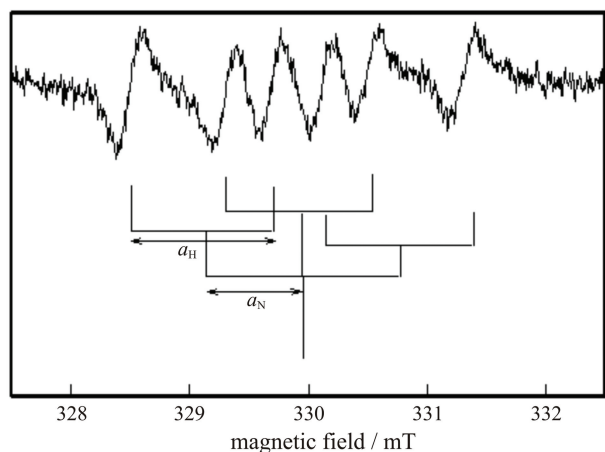
Figure 4. EPR spectrum of the aminocarbonylaminoxy radical ( \text{H}_2\text{N-CO-NHO}^\bullet ). Conditions: [\text{HU}] = 0.1 \text{ mol dm}^{-3} , [\text{Fe}(\text{CN})_6^{3-}] = 0.01 \text{ mol dm}^{-3} , [\text{HClO}_4] = 0.01 \text{ mol dm}^{-3} , at room temperature with f = 9.28 \text{ GHz} and 10 \text{ mW} .
