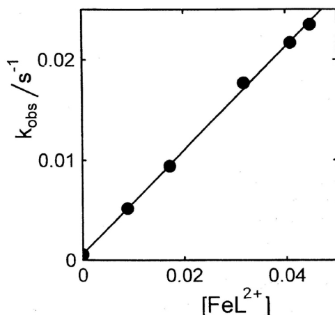
Figure 2. Dependence of the pseudo-first order rate constants for the formation of N -phenylformhydroxamic acid in the reaction of glyoxylic acid/glyoxylate with nitrosobenzene on the monoglyoxylato iron(III) complex concentration. 13 At pH = 1.56, in water, at 25 °C, ionic strength: 2.0 M (NaClO 4 /Fe(ClO 4 ) 3 ), total glyoxylate/glyoxylic acid: 0.05 M. Rate constants were determined as described earlier. 1a,b;2a,c Fraction of FeL 2+ complex was calculated (L - = glyoxylate) using an equilibrium quotient K_{eq} = 7.76 , defined as FeL^{2+} \cdot H^+ / Fe^{3+} \cdot HL for the formation of monoglyoxylato iron(III) complex, as determined spectrophotometrically, at pH = 1.56, (under the conditions employed in kinetic measurements, by measuring the increase of absorbance at 450 nm due to the formation of the complex).
