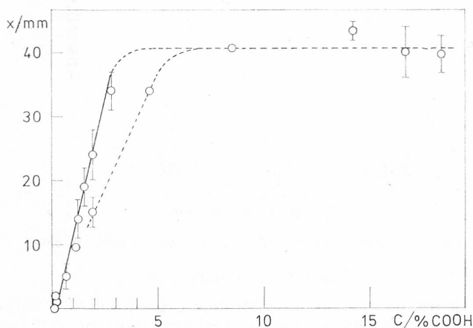
Figure 2. Calibration curve.
