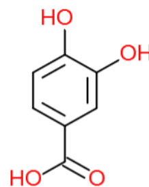
protokatehinska kiselina
