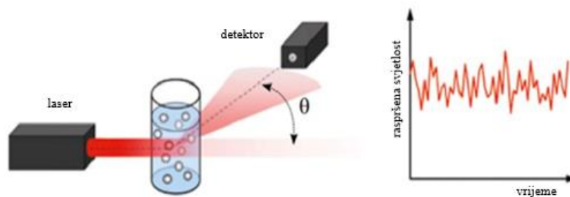
Slika 4. Princip dinamičkog raspršenja svjetlosti (preuzeto s https://wiki.anton-paar.com/en/the-principles-of-dynamic-light-scattering/##data-imagegroup-39782 )
