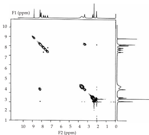
Fig. 2. The ^1\text{H} NOESY spectrum of TVA mesylate.
