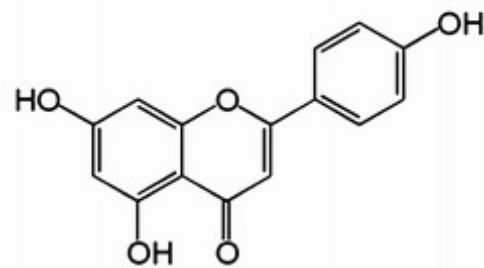
Apigenin
