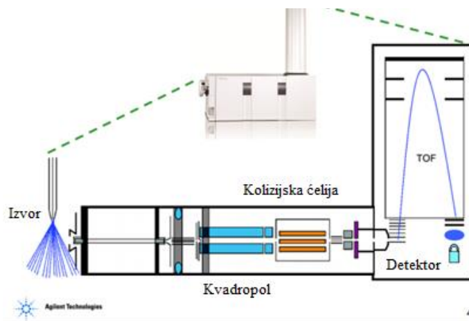
Slika 3: Q-TOF (Agilent Technologies, 2015)
