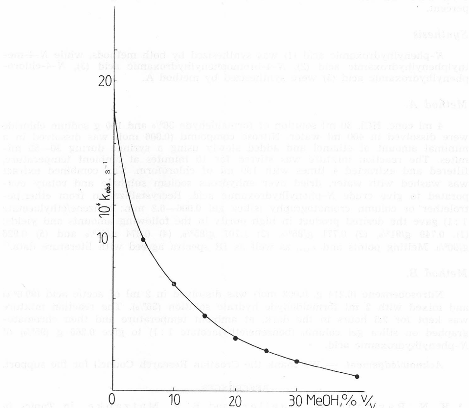
Figure 2. Dependence of rate constants for the reaction of formaldehyde with nitrosobenzene on the added methanol. Conditions: 0.688 M HCHO, 0.050 M \text{HClO}_4 , 2 M \text{NaClO}_4 , 25 °C. Rate constants were determined as described in Experimental.
